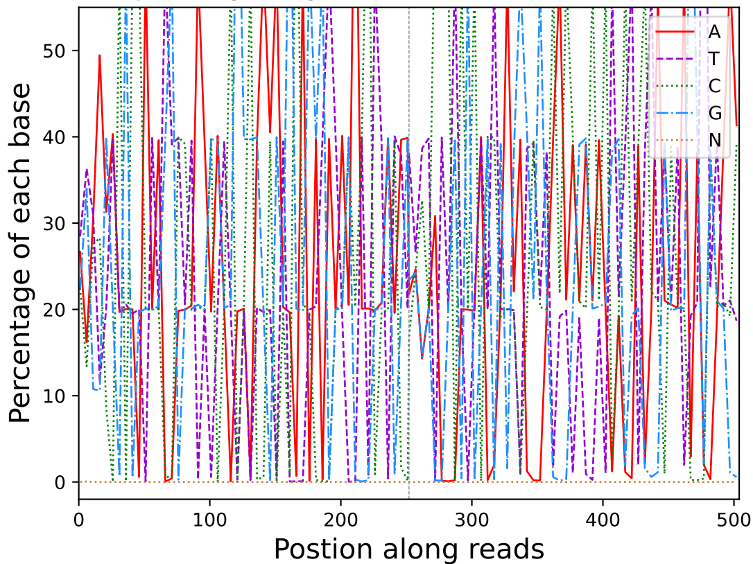
Base percentage along reads (R10410)
